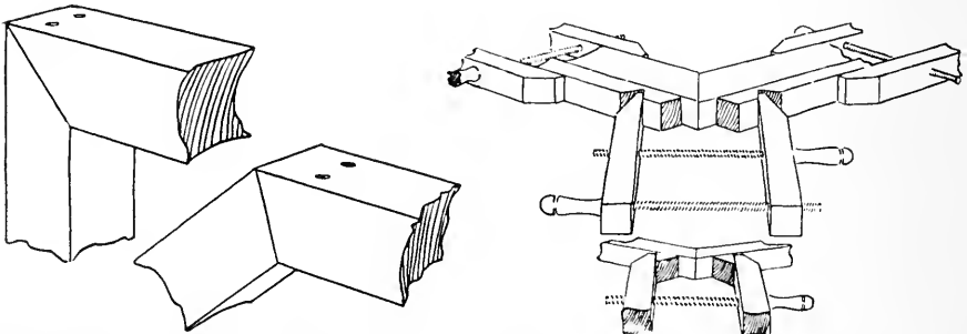
FIG. 264. PLAIN MITER JOINTS. FIG. 265. CLAMPING MITER JOINT.
